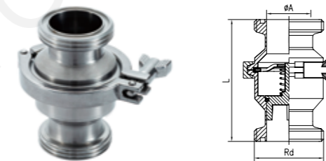
SMS check valve thread end
