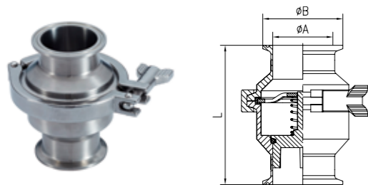
3A check valve clamp end
