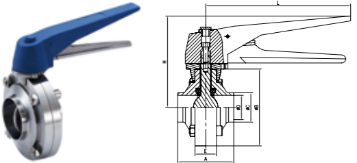
SMS butterfly valve weld end with gripper handle
