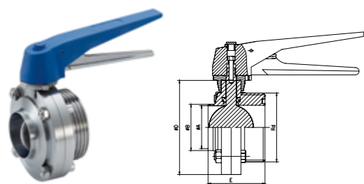
SMS butterfly valve weld/thread end with gripper handle
