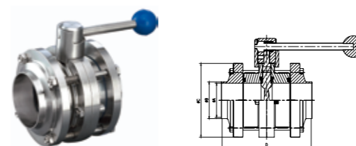
DIN 3PC butterfly valve weld end with pull handle
